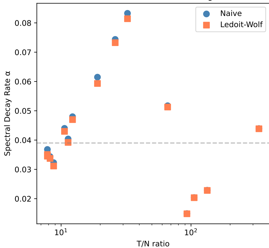
\alpha vs T/N: Naive vs Shrinkage
