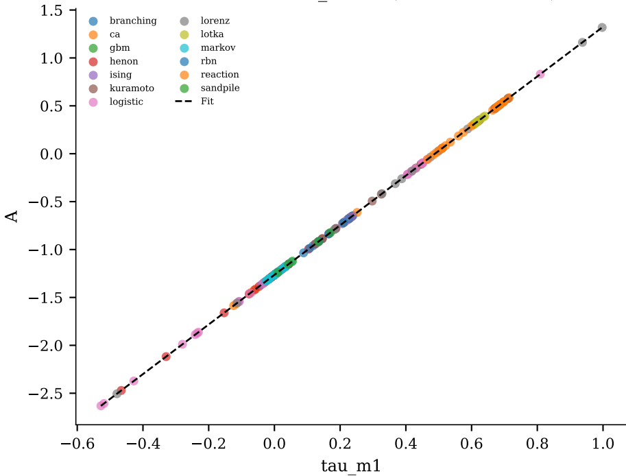
Best invariant: tau_m1 → A (linear, R^2=1.000 )
