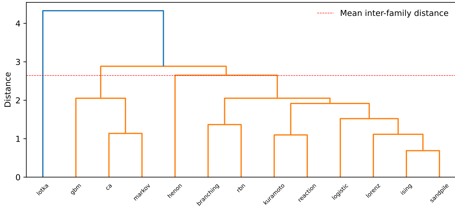
Family dendrogram (average linkage, centroid distance)
