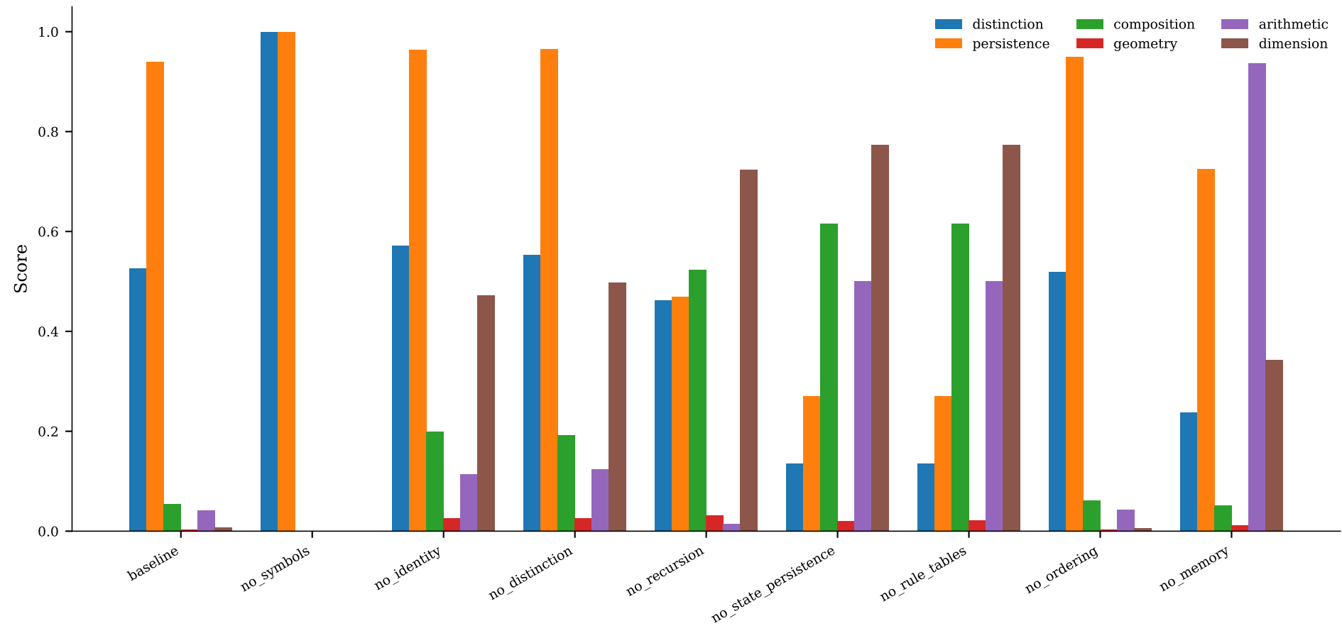
Emergence scores across ablation conditions
