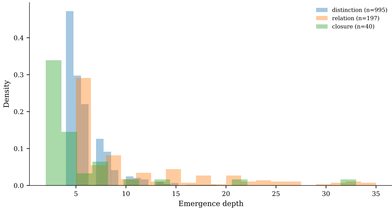
First emergence depths across properties
