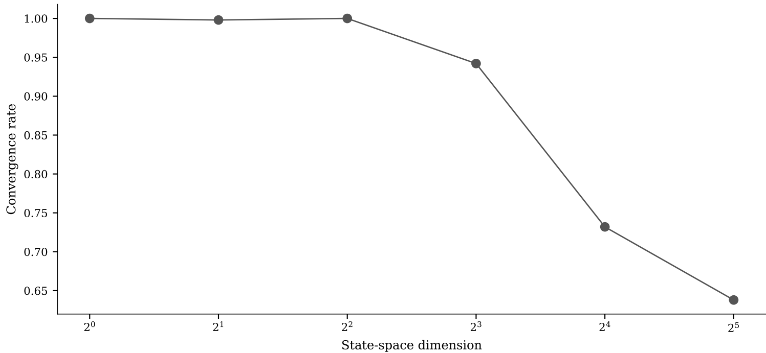
Convergence rate vs dimensionality
