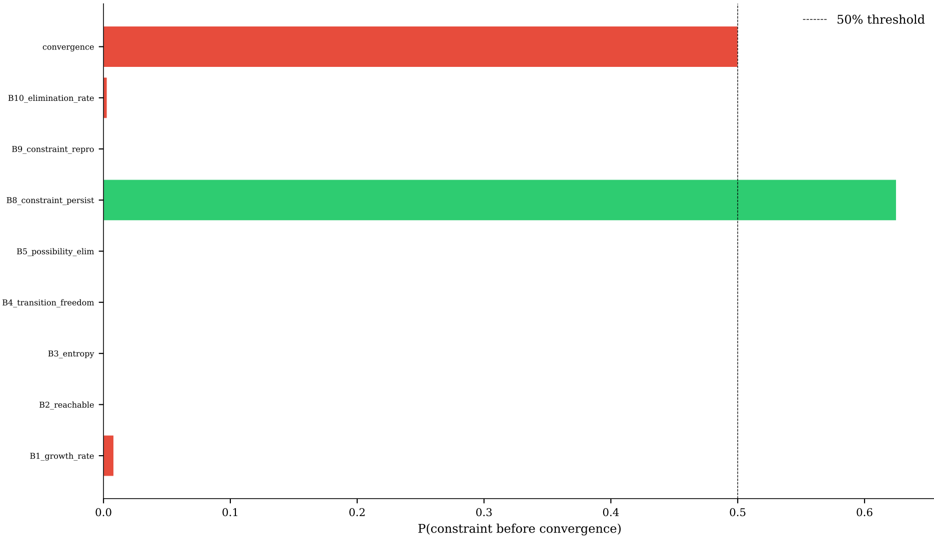
Pairwise order: constraint detectors vs convergence
