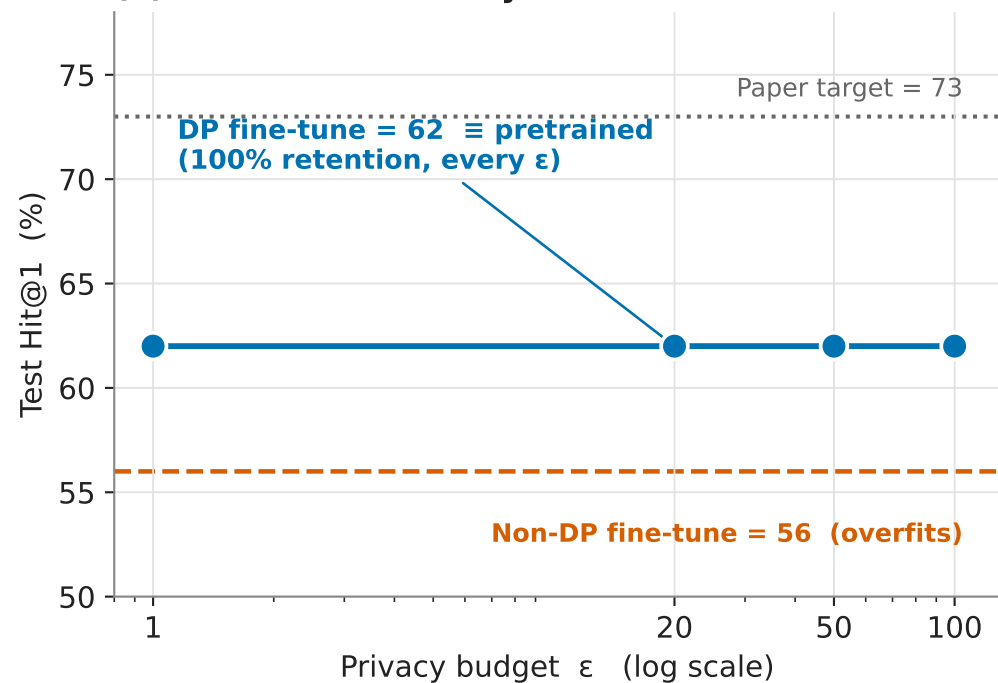
(a) Retrieval accuracy is flat across \epsilon
