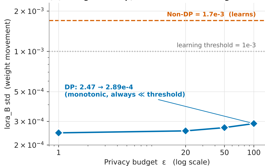
(b) Weights creep, never reach 'learning'
