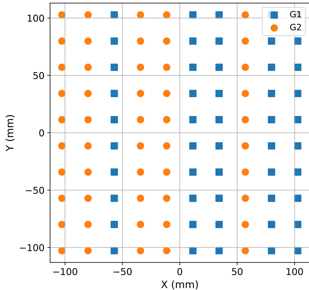
RIS Element Coordinates
