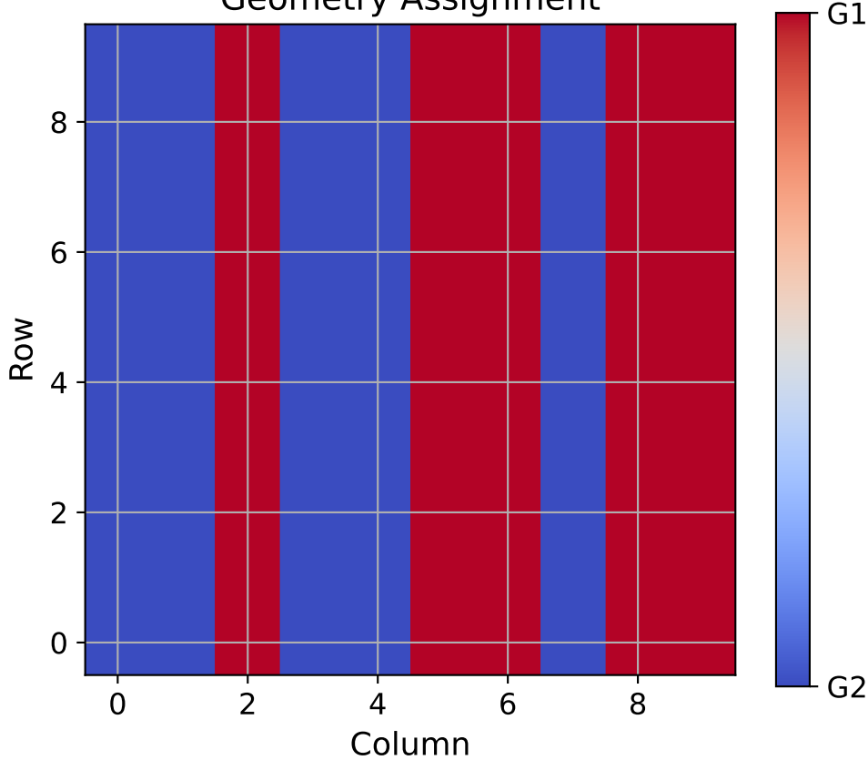
Geometry Assignment
