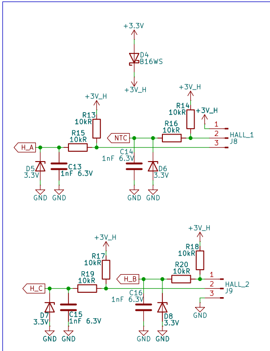
Hall Sensors
