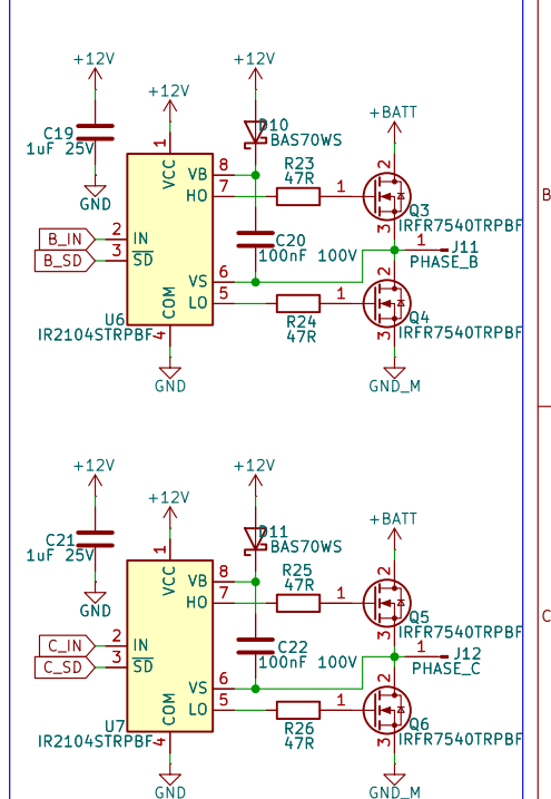
Drivers
