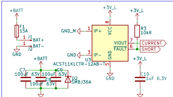
Protection
