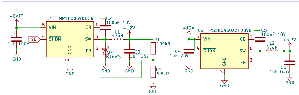
Converters
