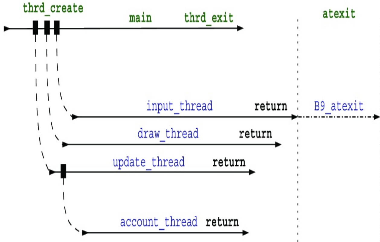
Figure 20.4 Control flow of the five threads of B9-detach. The thread that returns last executes the atexit handlers.
