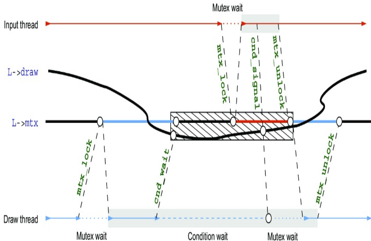
Figure 20.3 Control flow managed by mutex L->mtx and condition variable L->draw between the input and draw threads. Critical sections are shaded with grey. The condition variable is associated with the mutex until the waiter has reacquired the mutex.
