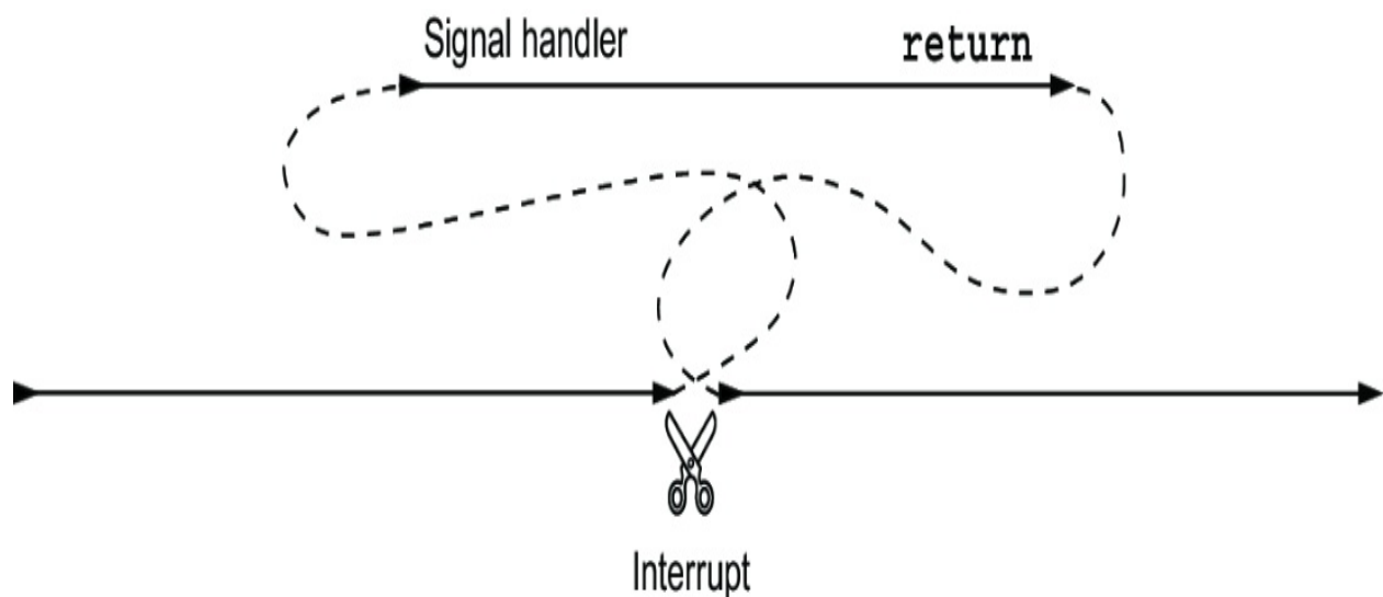
Figure 19.3 Control flow after an interrupt return jumps to the position where the interrupt occurred
