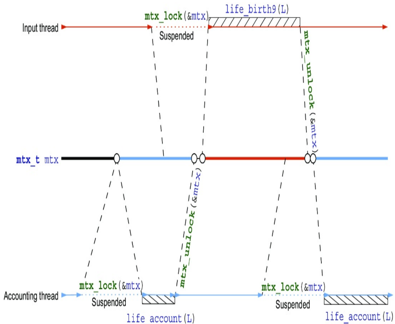
Figure 21.2 Two threads with three critical sections that synchronize via a mutex. The circles present the modifications of object mtx .
