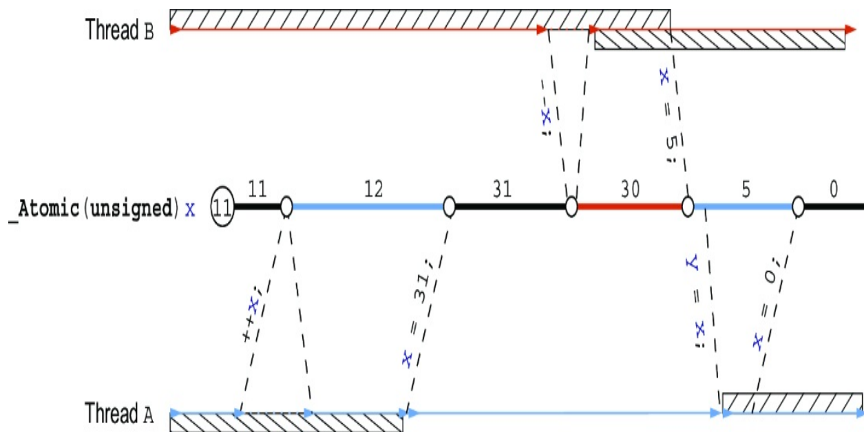
Figure 21.1 Two threads that synchronize via an atomic. The circles present the modifications of object x . The bars below the threads represent information about the state of A, and those above represent information about the state of B.
