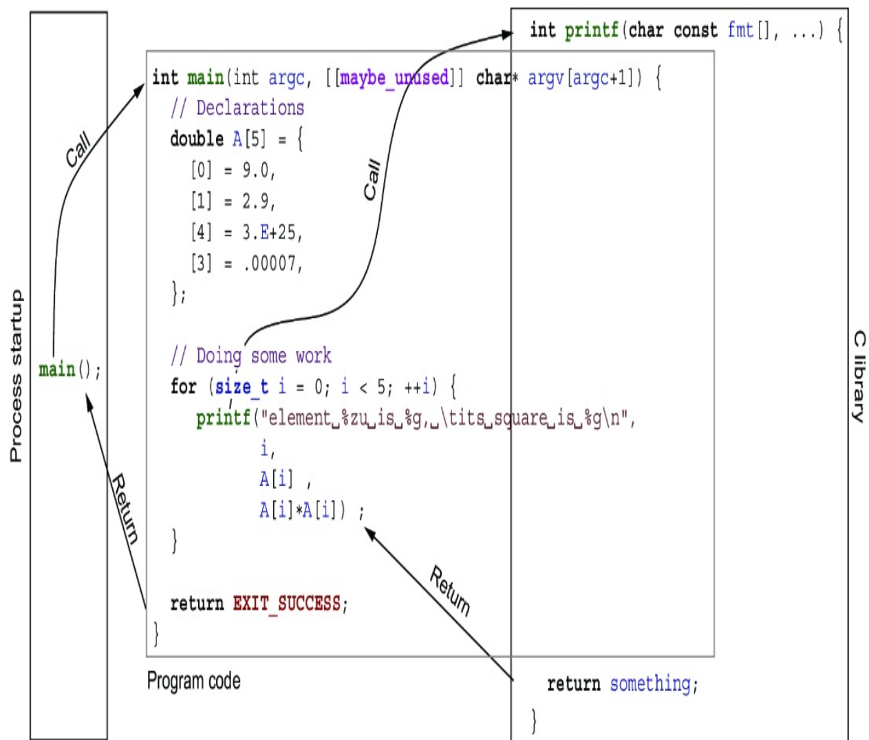
Figure 2.1 Execution of a small program
