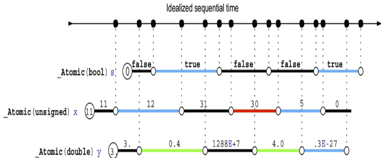
Figure 21.3 Sequential consistency for three different atomic objects
