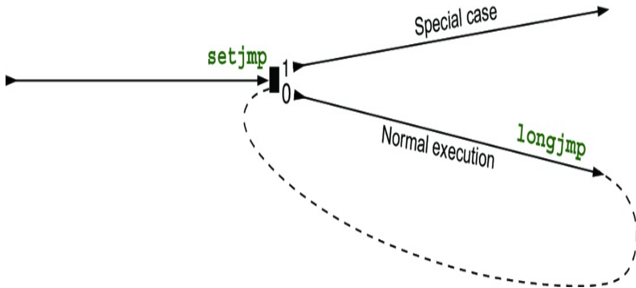
Figure 19.2 Control flow with setjmp and longjmp : longjmp jumps to the position marked by setjmp .
