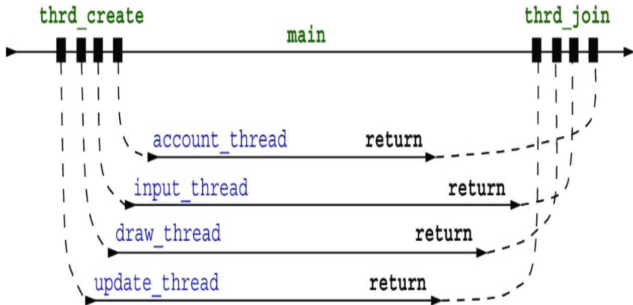
Figure 20.1 Control flow of the five threads of B9
