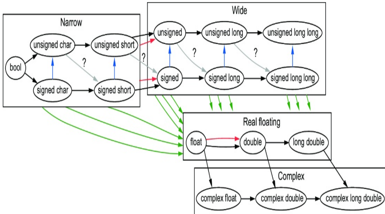
Figure 18.1 Upward conversion of some standard arithmetic types. Black arrows conserve values; red arrows (between narrow and wide types) may occur for integer promotion or default argument conversion; blue arrows (from signed to unsigned types) are reduction modulo 2^N ; well-definition of gray arrows (with question marks) depends on the platform; green arrows (from integers to floating types) may lose precision.
