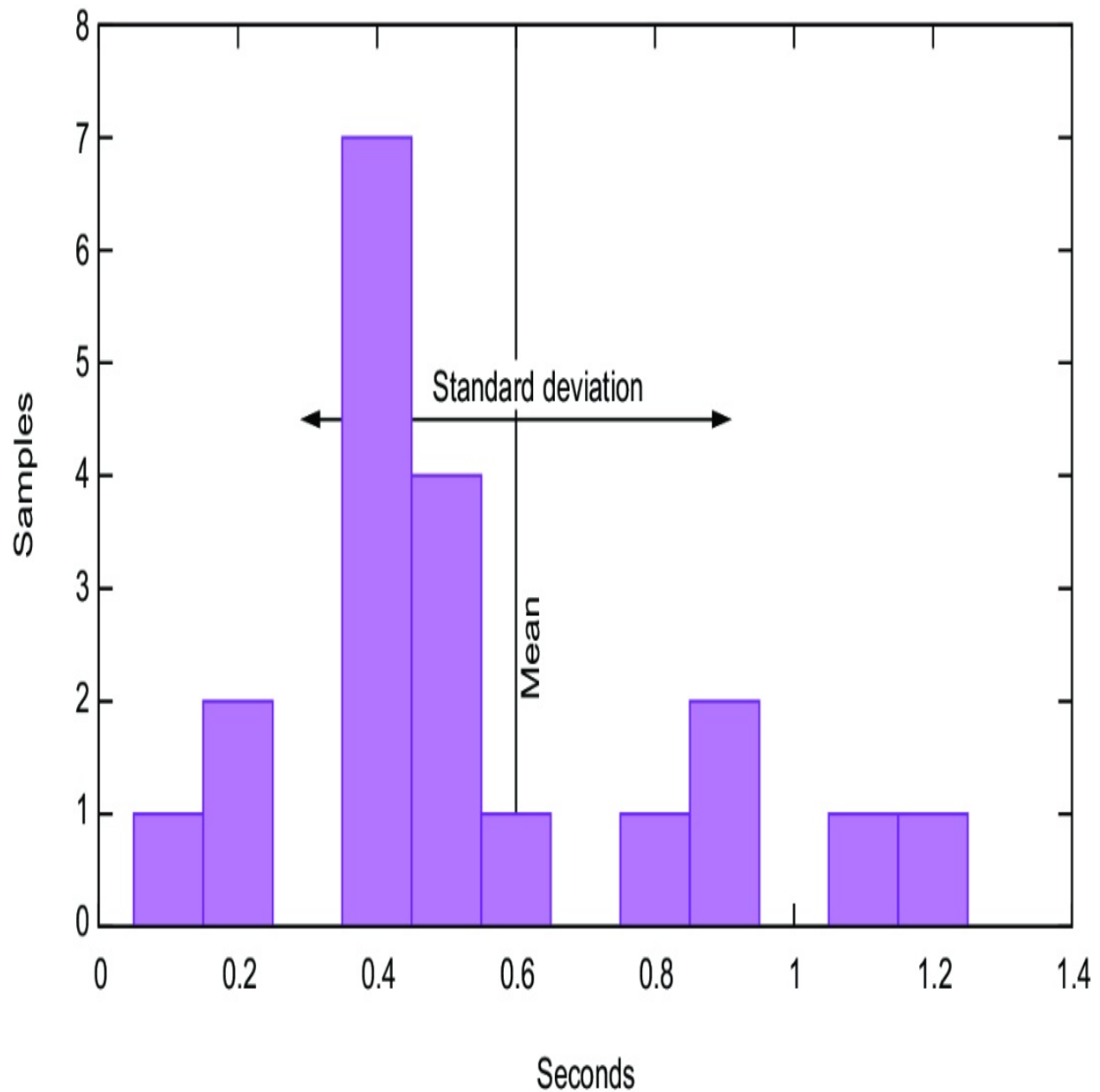
Figure 16.1 Frequency histogram for our sample, showing the frequency with which each of the measured values was obtained
