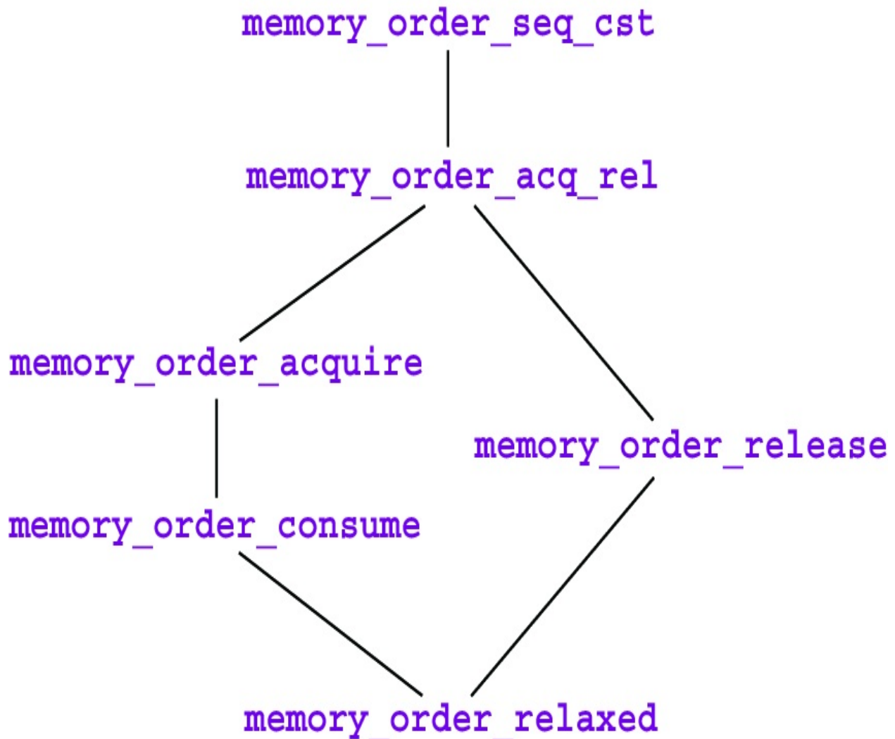
Figure 21.4 Hierarchy of consistency models, from least to most constraining
