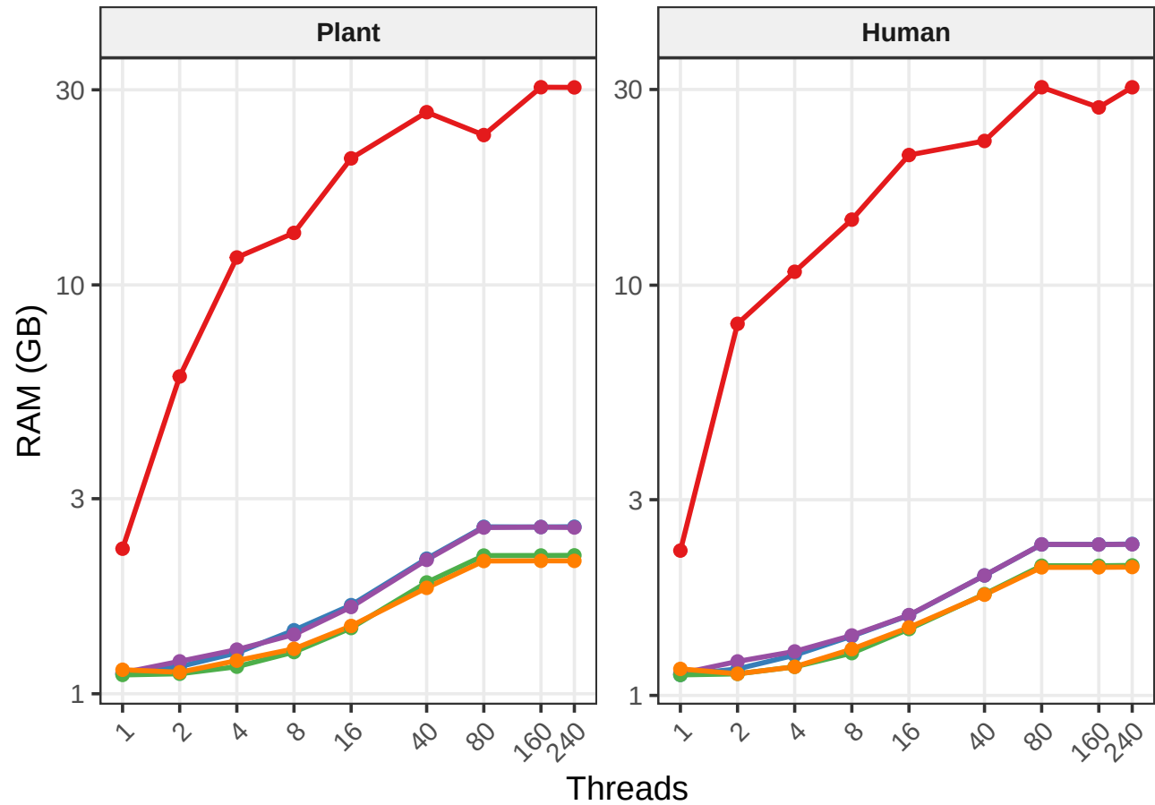
B. Peak Memory Usage
