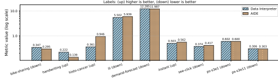
Figure 16: Comparison between Data Interpreter and AIDE on nine Kaggle-style competition datasets with valid results from both agents.
