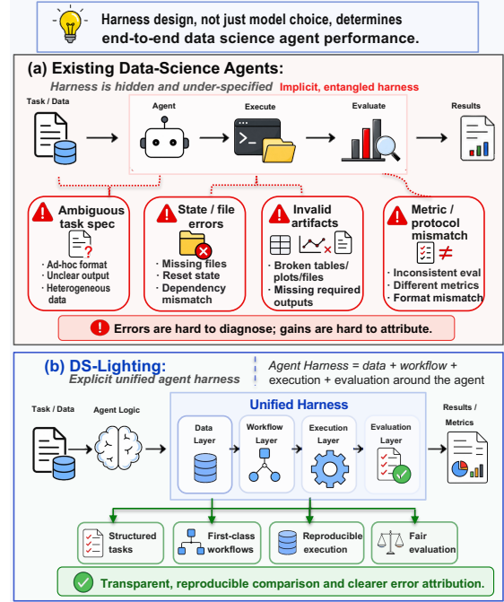
Figure 1: Existing data-science agents vs. DS-Lighting (ours). The contrast motivates a harness-centered design: existing agents entangle task data, execution, and evaluation, while DS-Lighting decouples them to ground data, govern execution, and align outputs with metrics.
