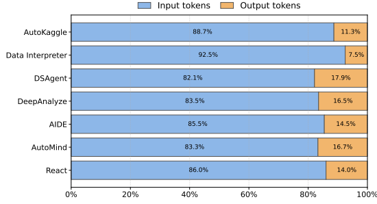
Figure 13: Input/output token composition of different agents.
