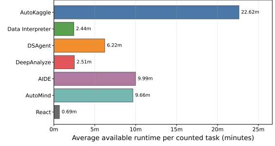
Figure 14: Average running time of different agents.
