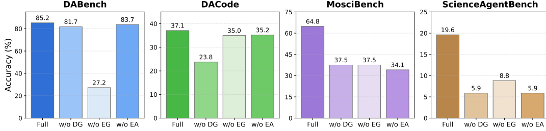
Figure 3: Ablation of DS-Lighting’s system-level mechanisms.
