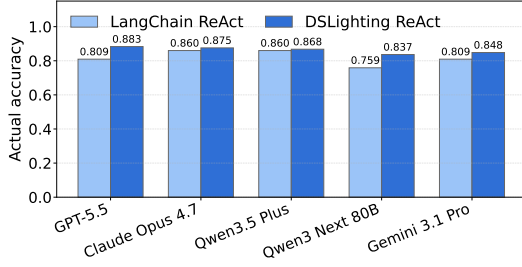
Figure 4: Performance across different models.
