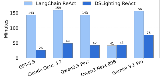
Figure 15: Runtime comparison between LangChain ReAct and DS-Lighting ReAct across models on DABENCH.
