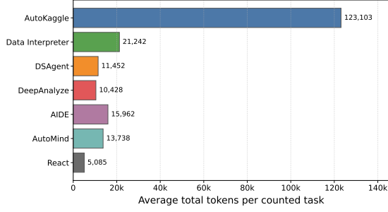
Figure 12: Average token consumption of different agents.
