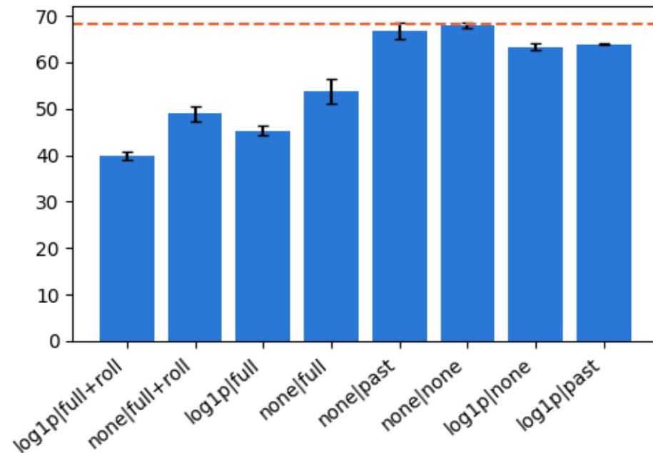
MAE: mean over seeds ( \pm seed std)
