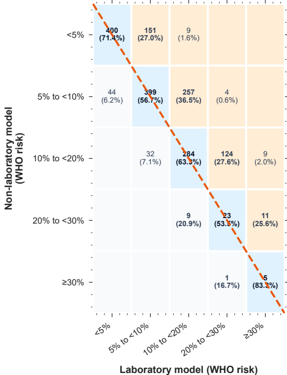
Cross-classification Heatmap
