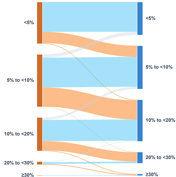
Individual-level Reclassification Migration Non-laboratory Model Laboratory Model
