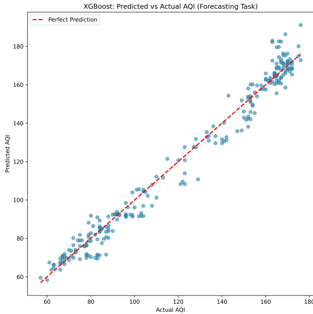
Fig. 3. Predicted vs. actual AQI values for the XGBoost forecasting model.
