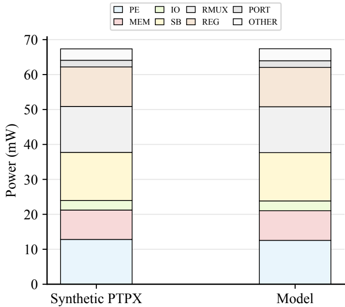
(b) Power breakdown.
