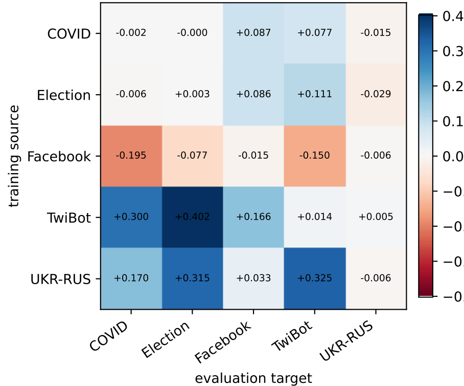
NM+MT – MT ROC-AUC
