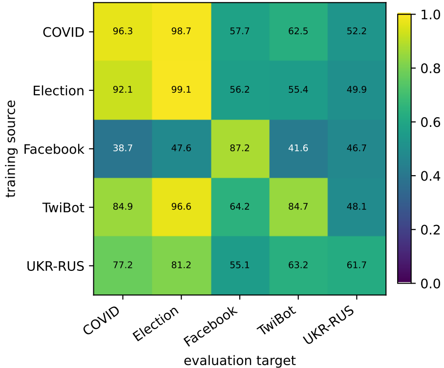
NM+MT ROC-AUC (%)
