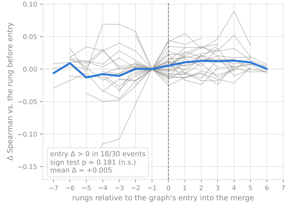
Node regression
