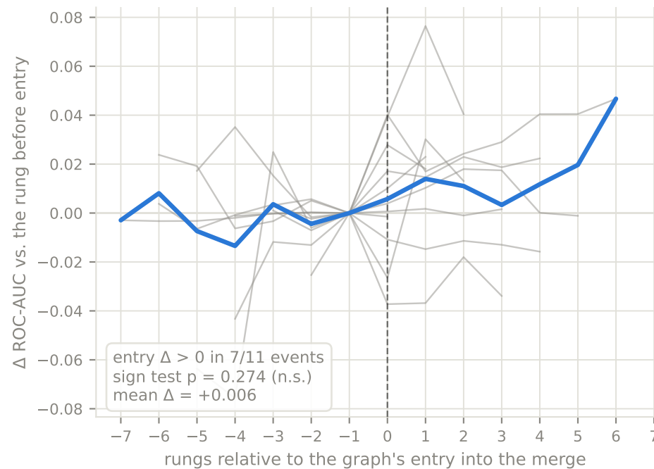
Node classification
