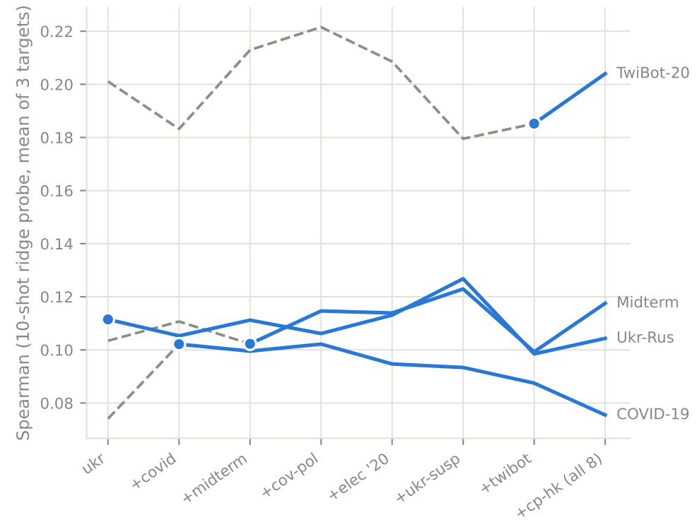
Node regression
