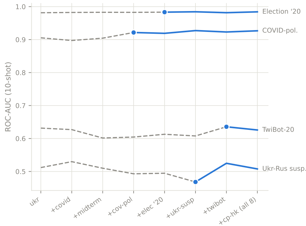
Node classification
