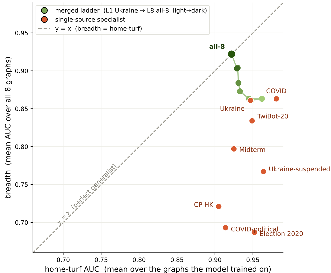
Generalist vs specialist — NM (3-shot / 30-way, matched-40k)
