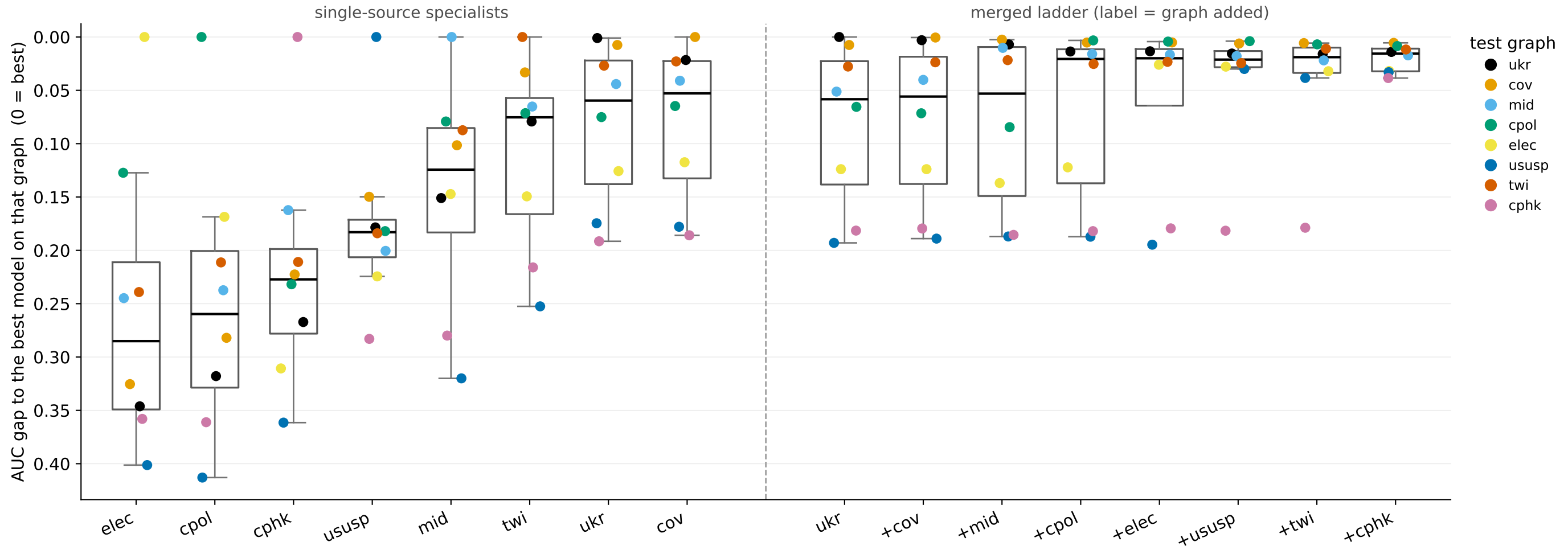
How far each model trails the best on each test graph — specialists vs ladder (best over all 16 models; single-source by mean gap worst→best; ladder in entry order; 1 seed)
