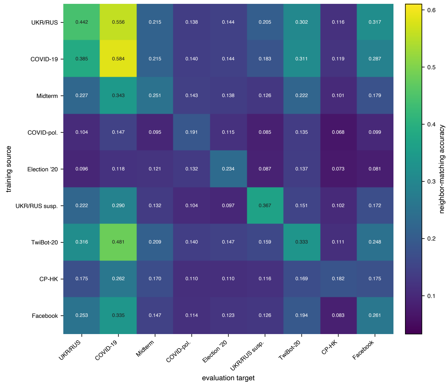
PRODIGY matrix · training seed 2
