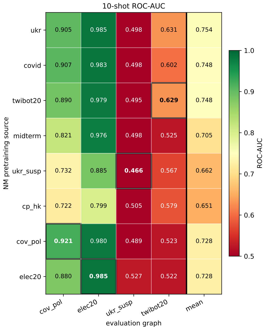
Node classification transfer of eight single-source NM encoders rows follow NM donor-strength order · outlined cells are in-domain
