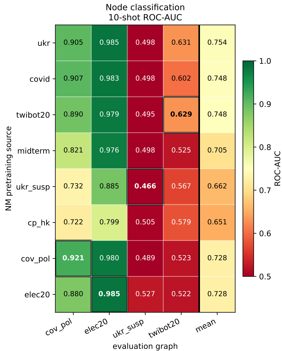
Downstream transfer of eight single-source NM encoders rows follow NM donor-strength order · outlined cells are in-domain
