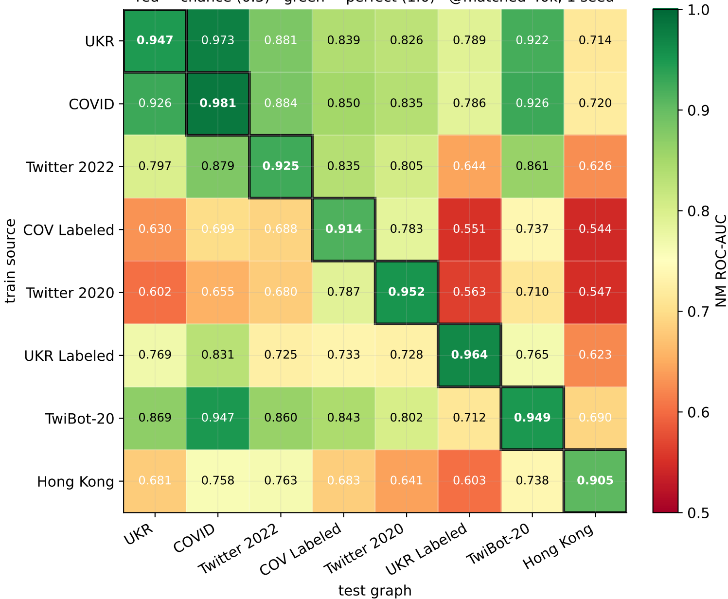
Single-source NM transfer matrix (ROC-AUC) red = chance (0.5) · green = perfect (1.0) · @matched-40k, 1 seed
