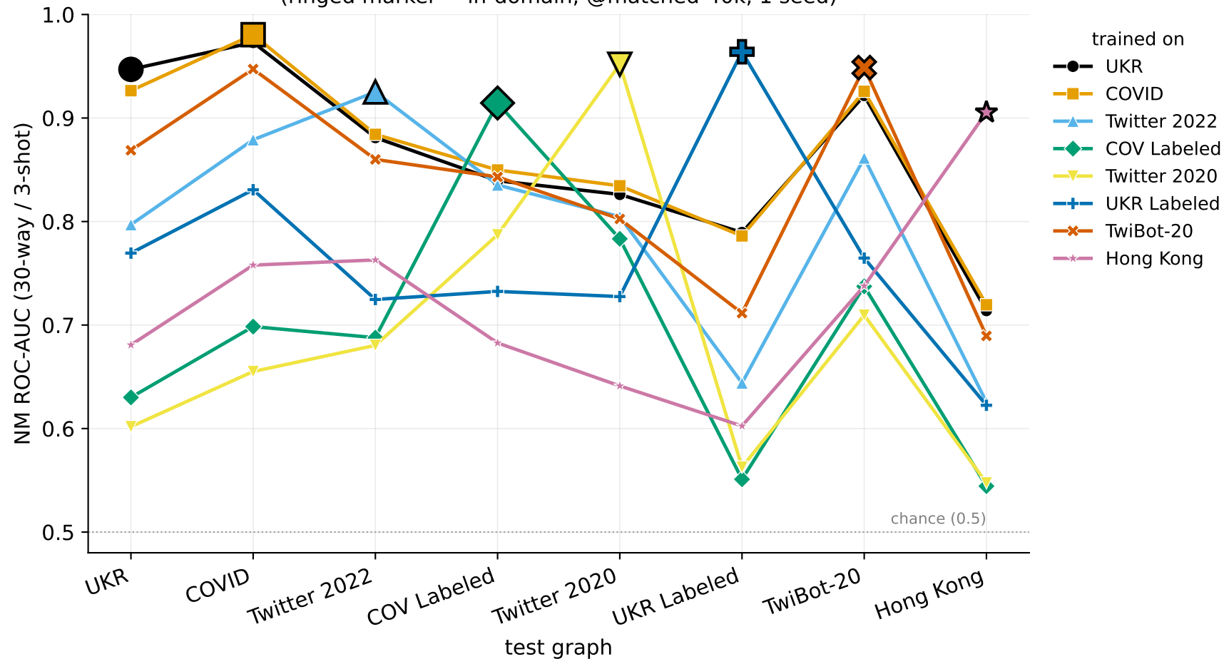
Single-source NM: each specialist's AUC profile across all test graphs (ringed marker = in-domain; @matched-40k, 1 seed)
