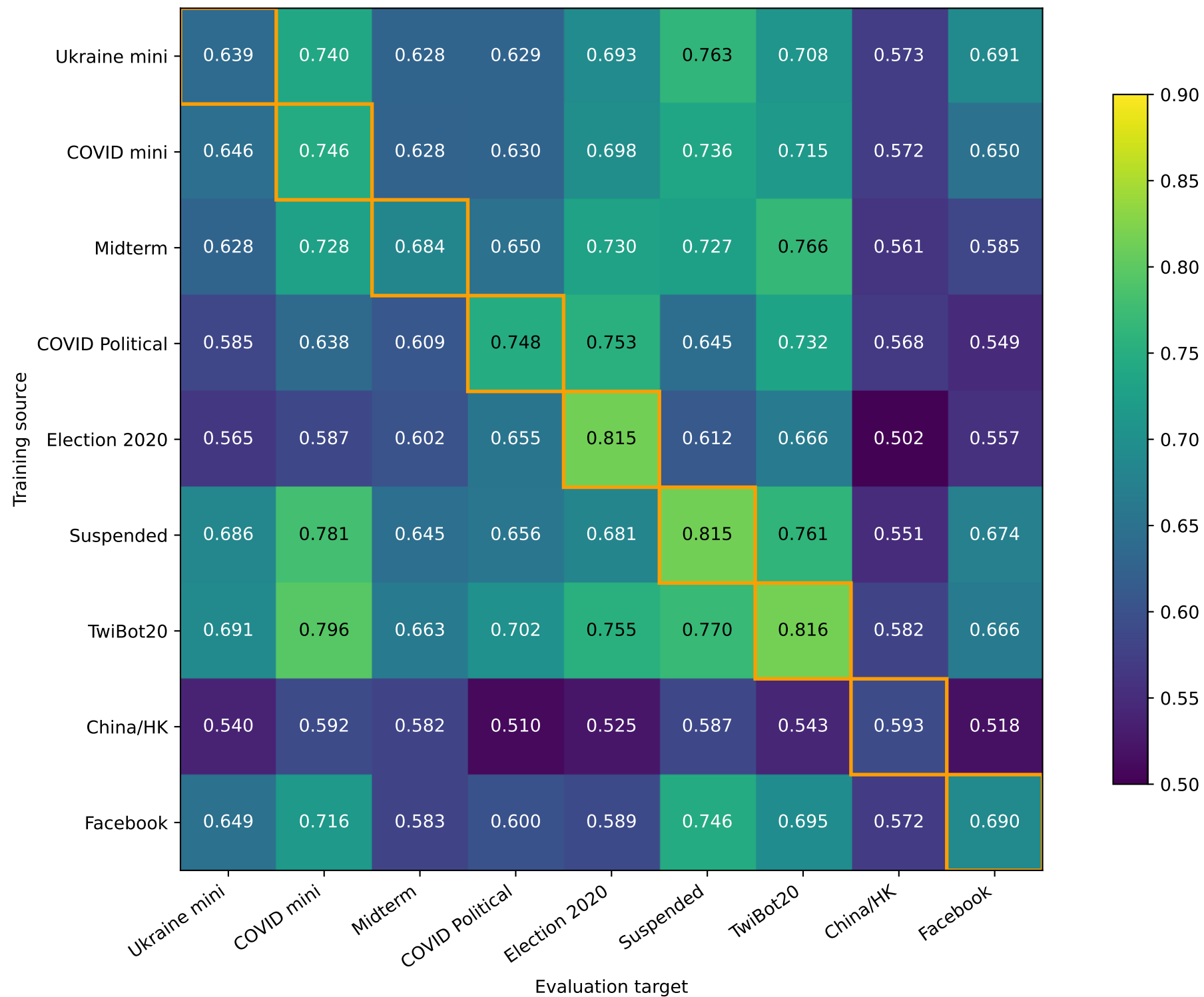
Node + 10-neighbor LP • raw-dot AUC ↑
