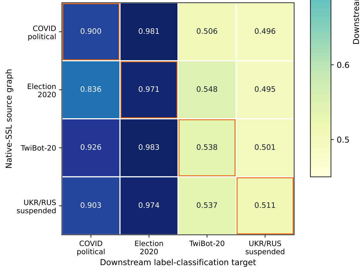
GraphSAGE · edge negative sampling step 2,500 · 1 seed
