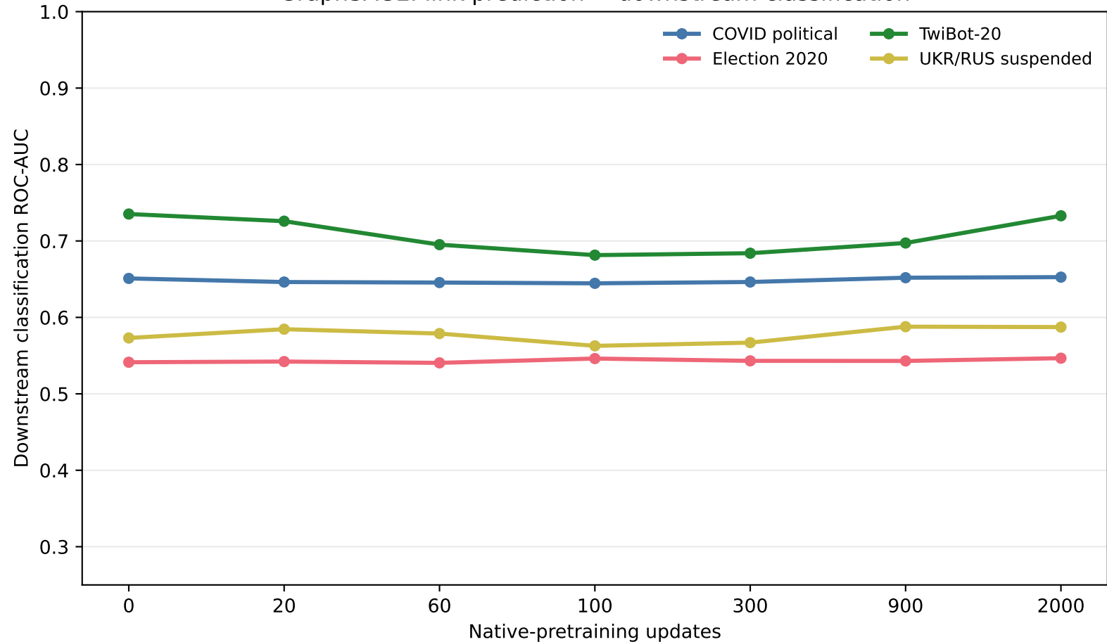
GraphSAGE: link prediction → downstream classification
