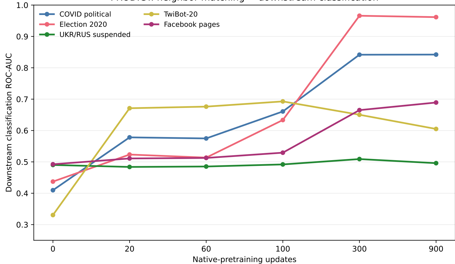
PRODIGY: neighbor matching → downstream classification
