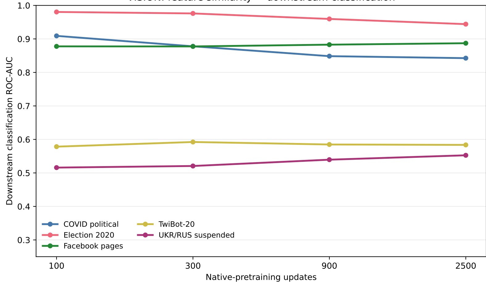
VISION: feature similarity \rightarrow downstream classification
