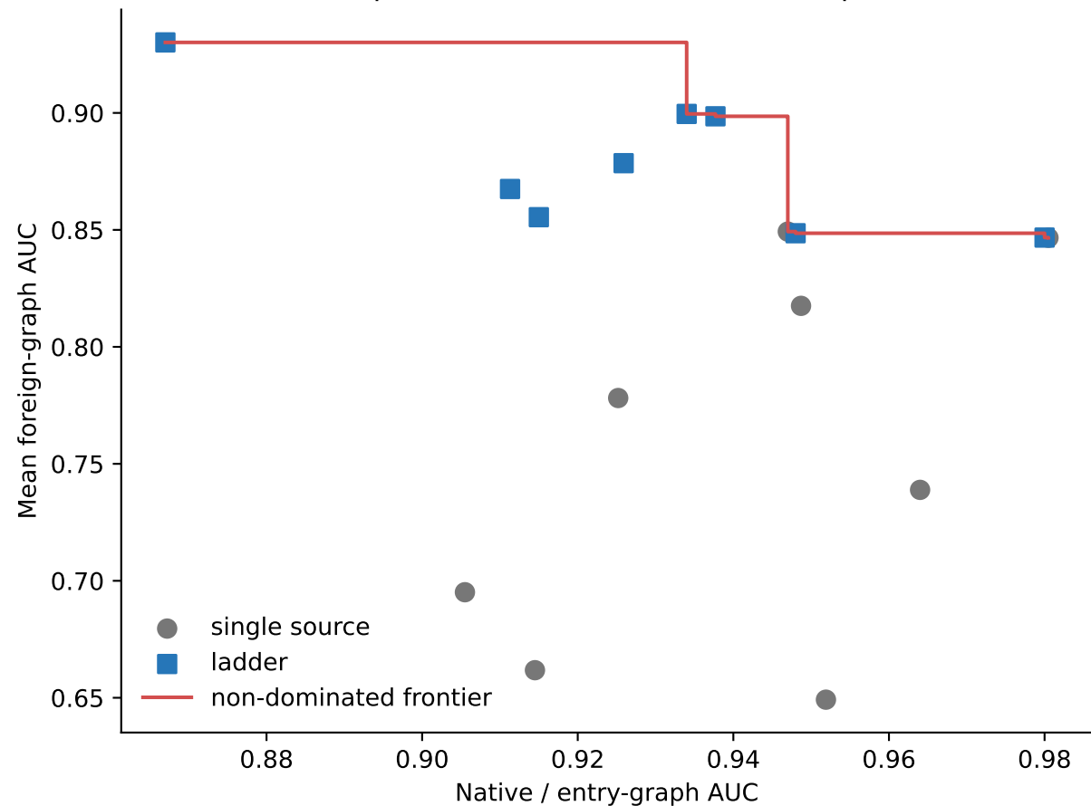
Specialization-breadth Pareto map
