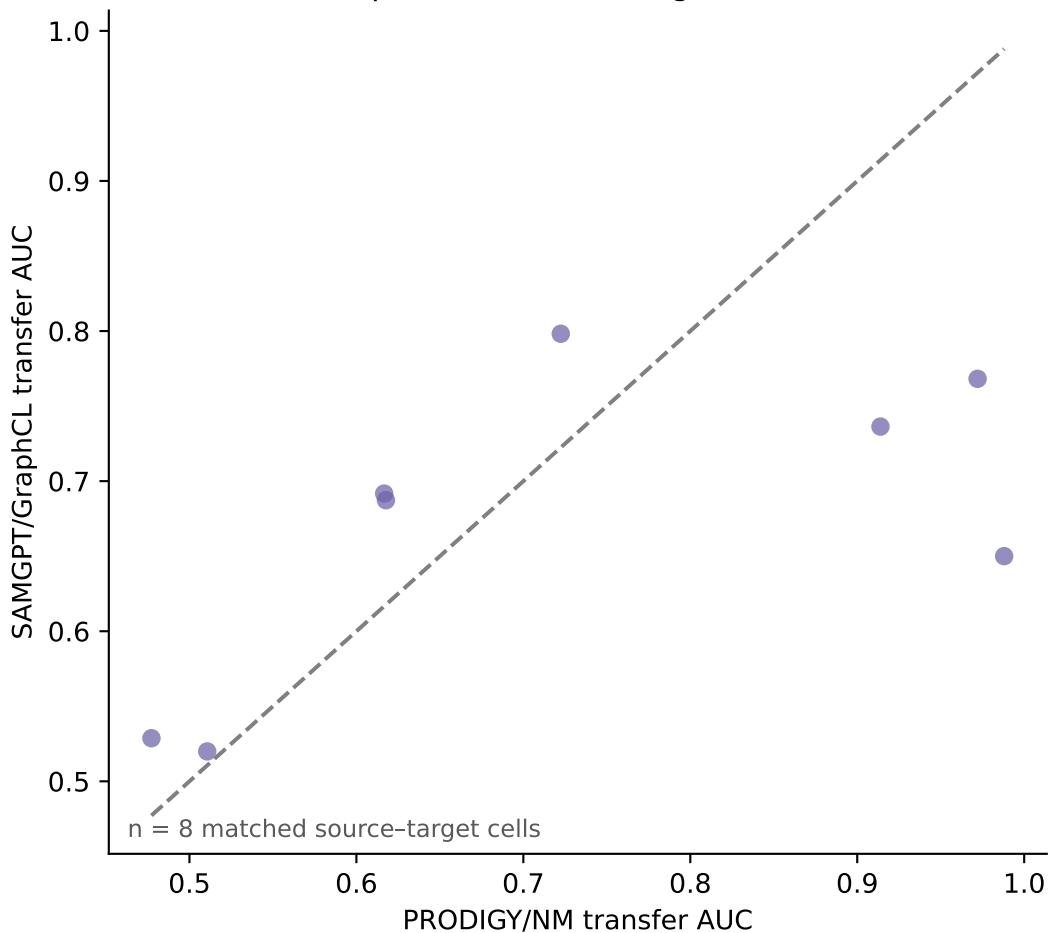
Cross-model pairwise transfer agreement ( r = 0.64 )
