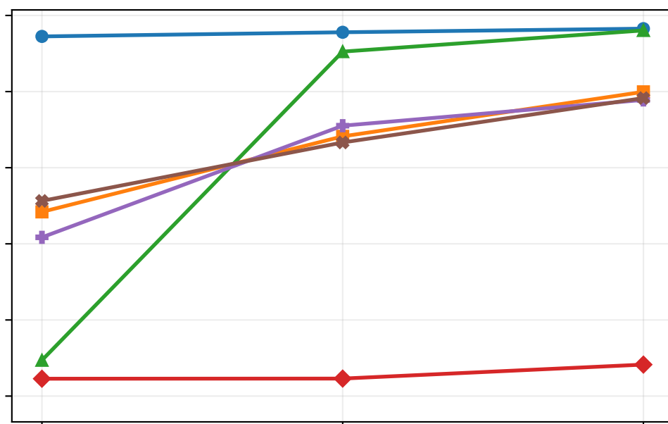
d TwiBot-20
