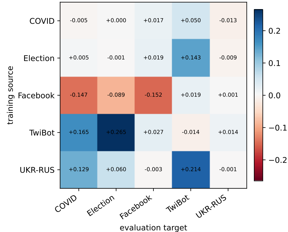
NM+MT – MT accuracy
