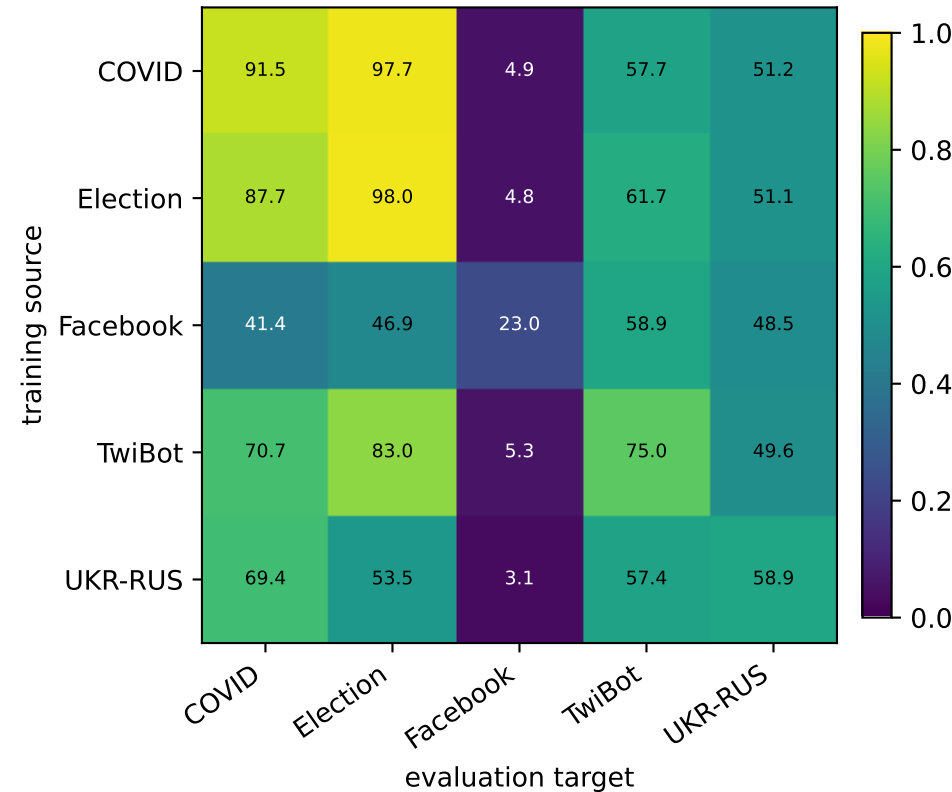
NM+MT accuracy (%)
