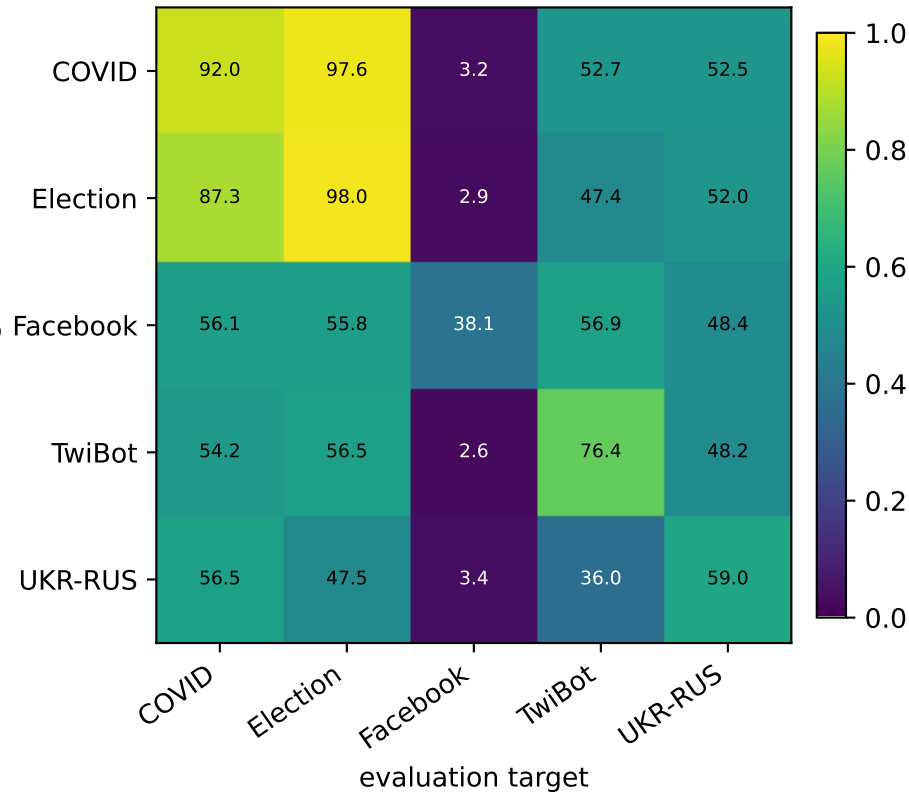
MT accuracy (%)
