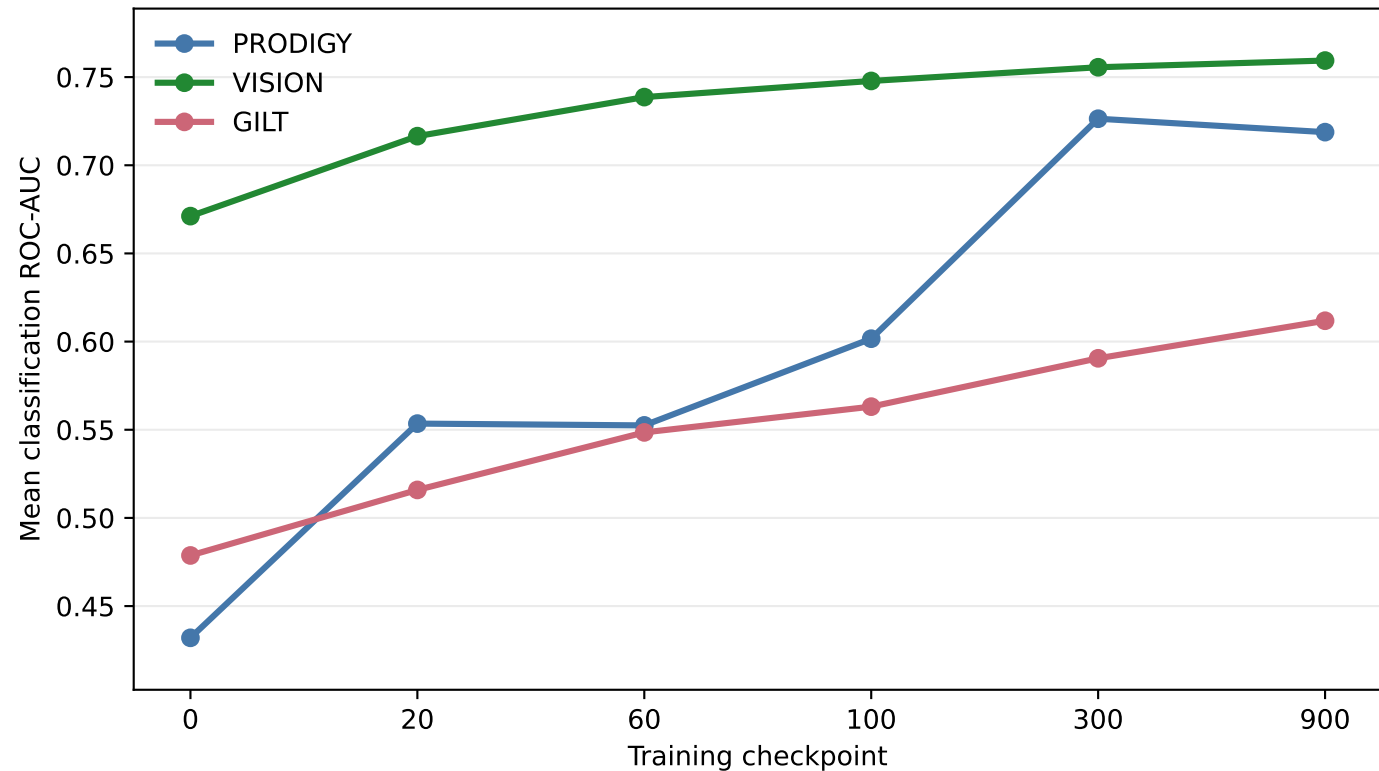
Native-objective training: classification transfer
