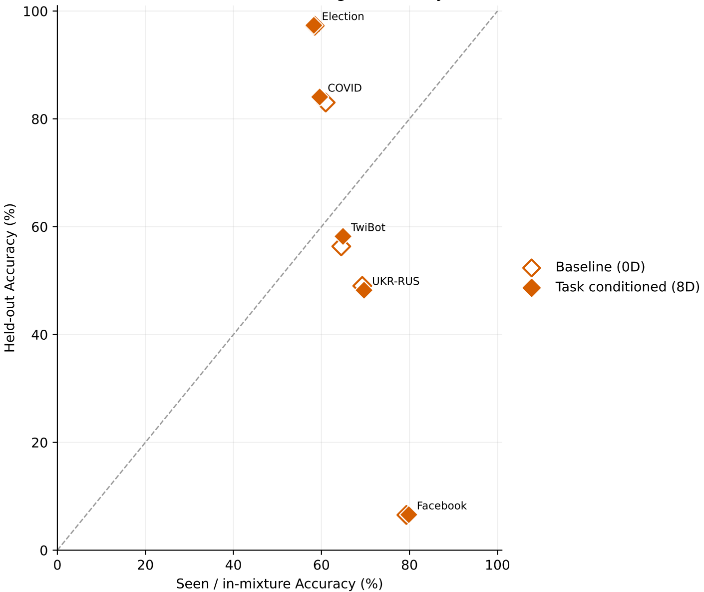
NM+MT 8D task conditioning — Accuracy
