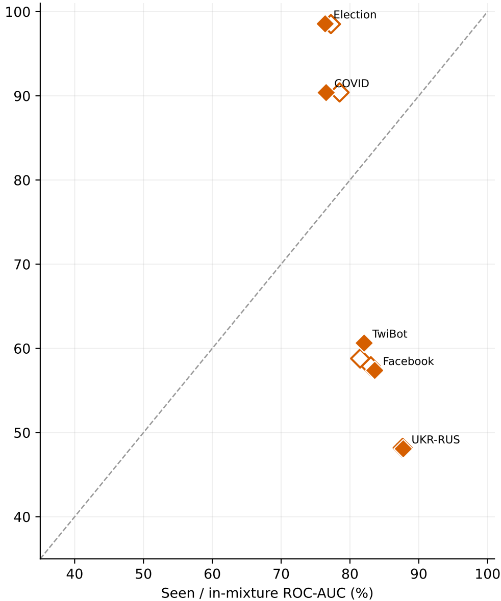
NM+MT 8D task conditioning — ROC-AUC
