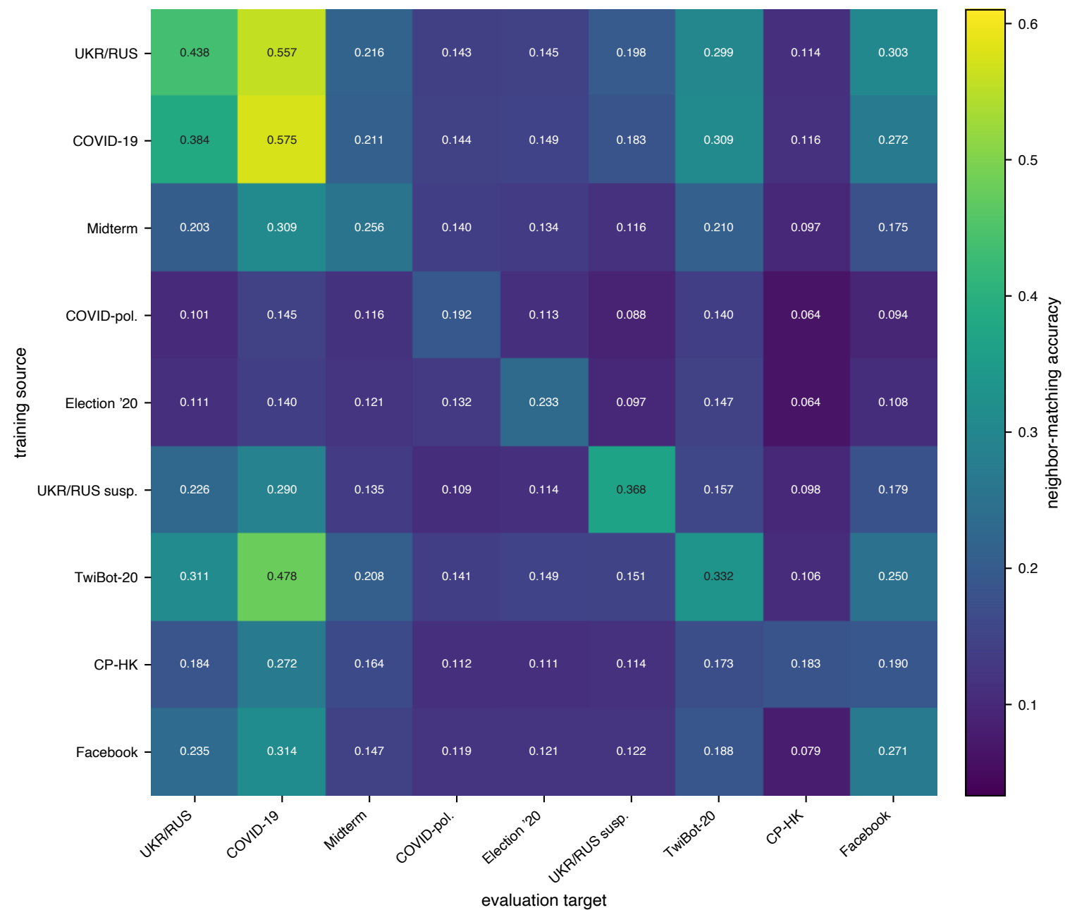
PRODIGY matrix · training seed 1
