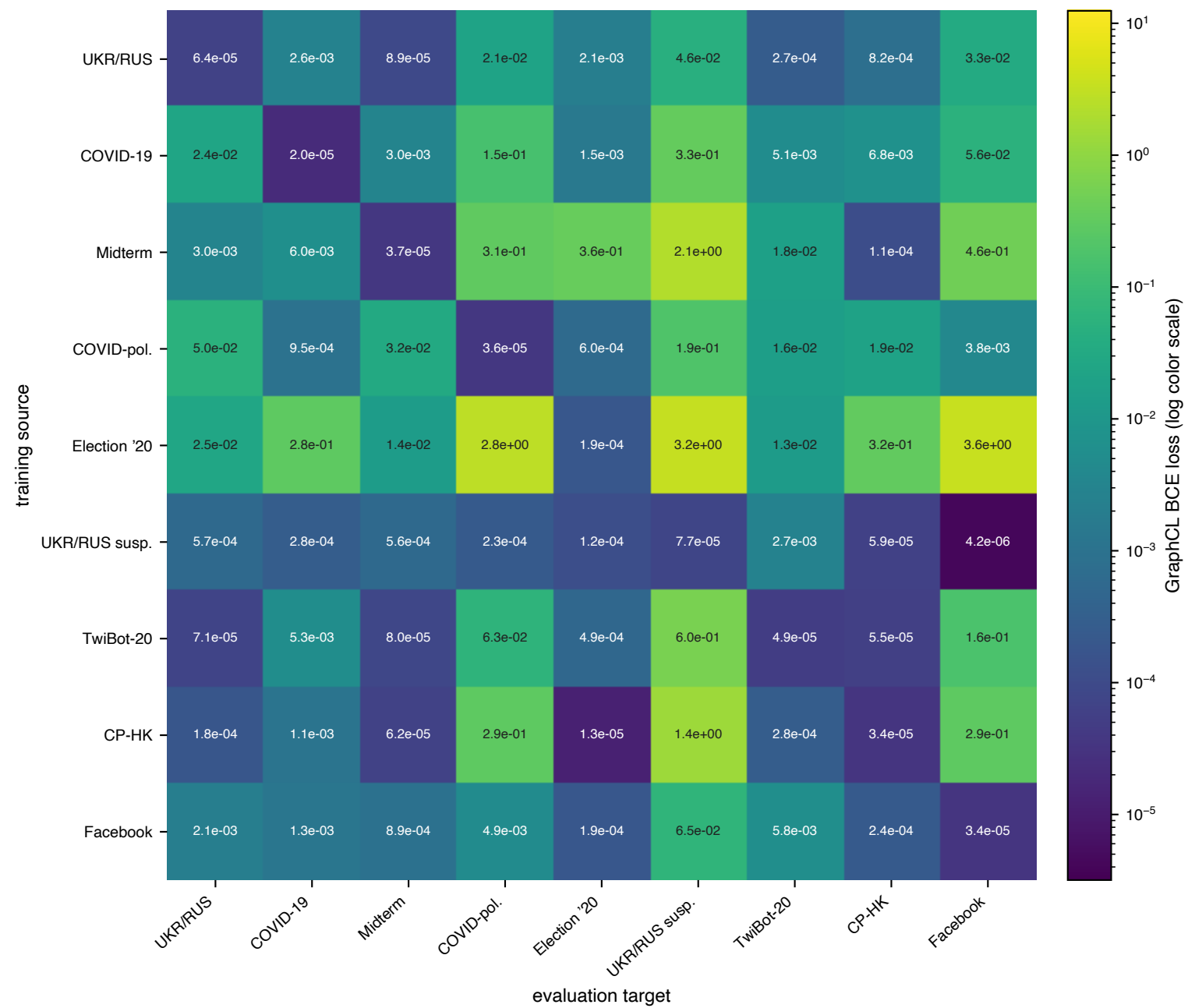
SAMGPT matrix · training seed 40
