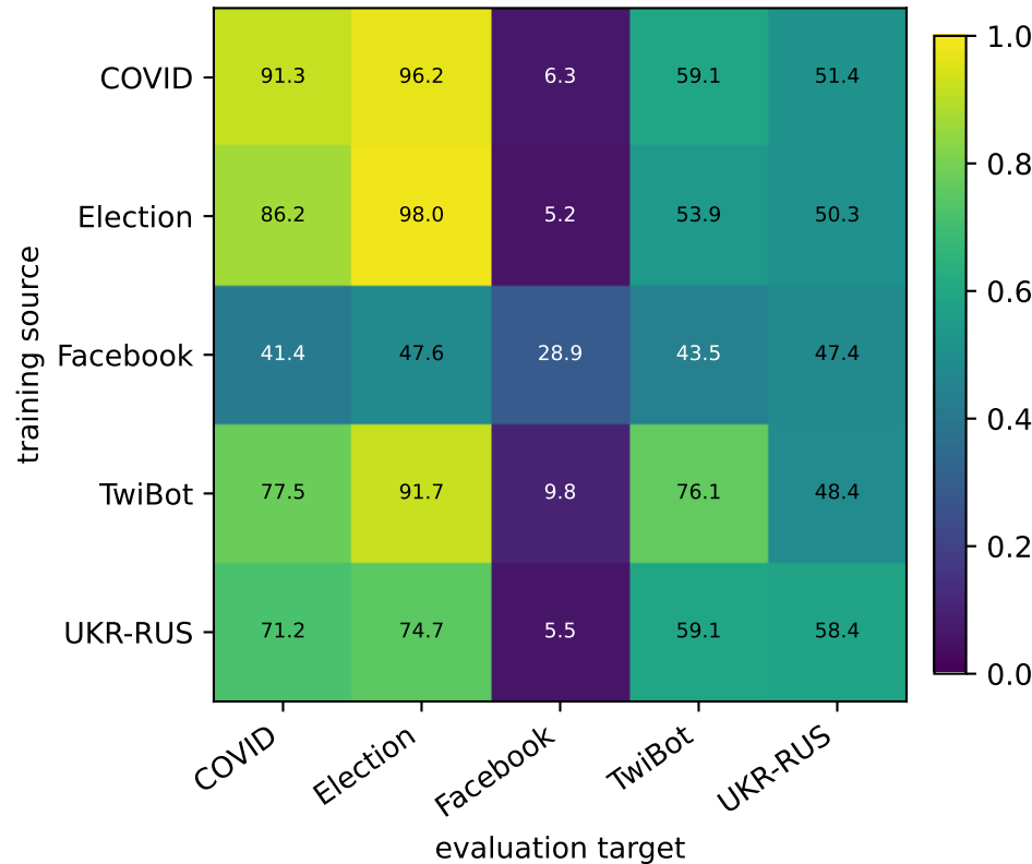
NM+MT accuracy (%)
