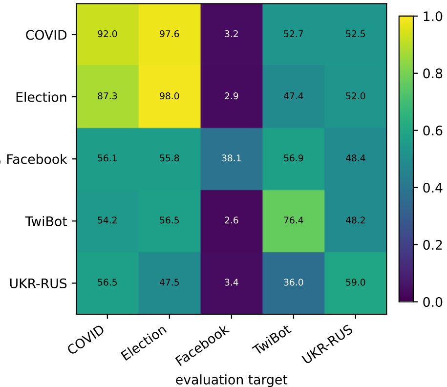
MT accuracy (%)
