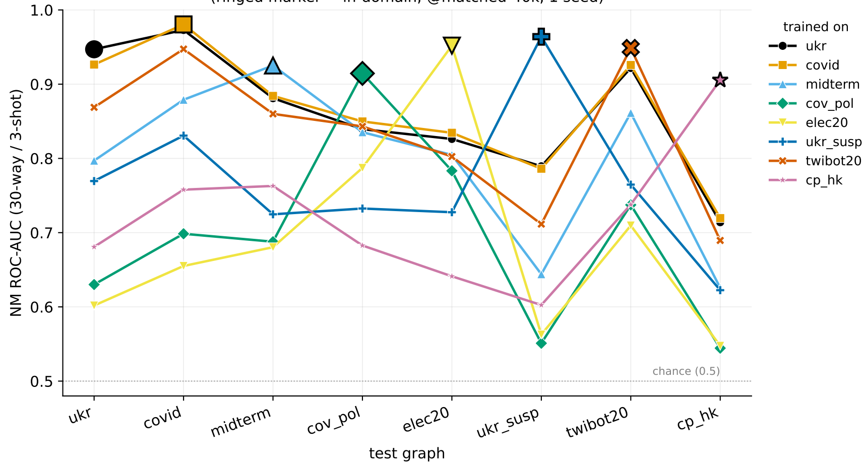
Single-source NM: each specialist's AUC profile across all test graphs (ringed marker = in-domain; @matched-40k, 1 seed)
