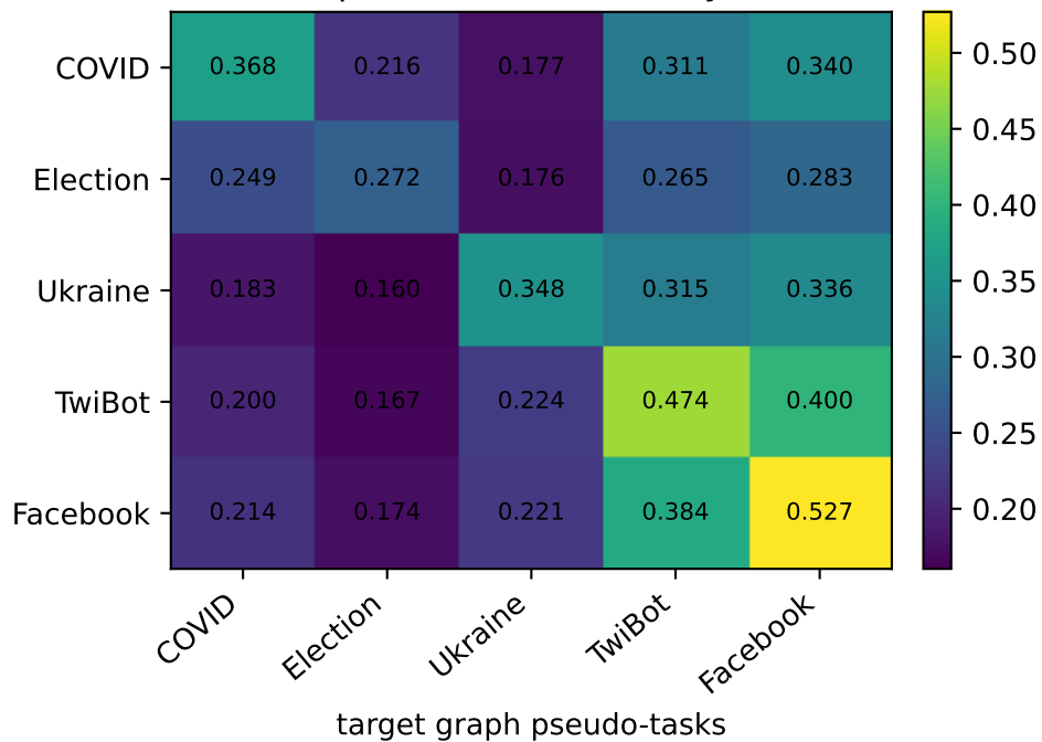
pseudo-task accuracy
