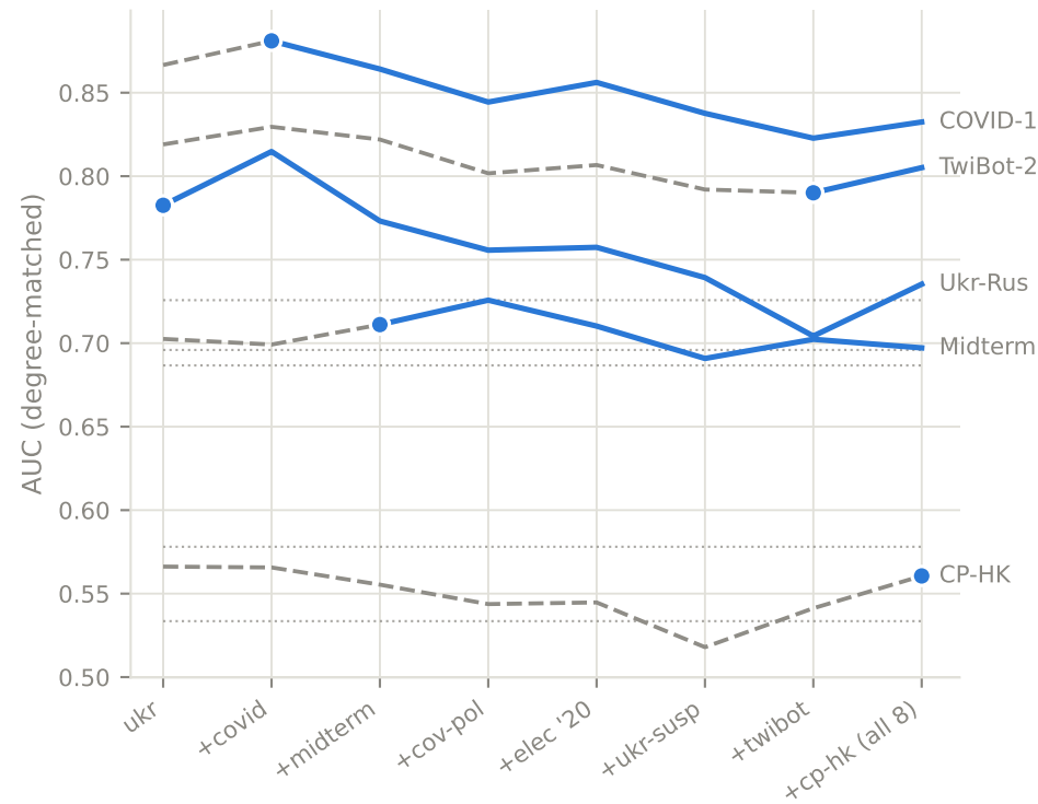
Static link prediction
