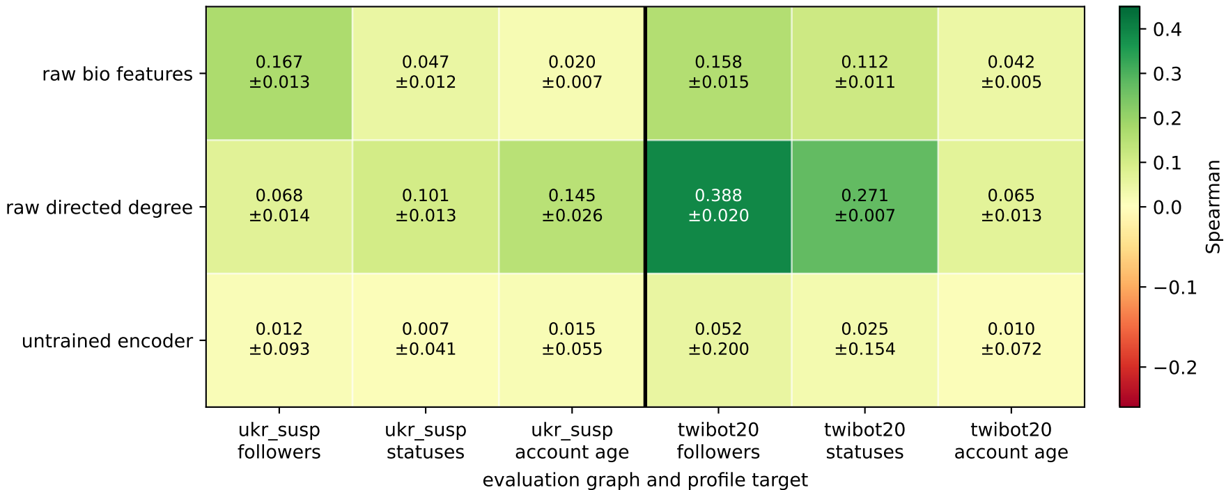
10-shot node-regression floors mean Spearman \pm sample SD across 5 seeds
