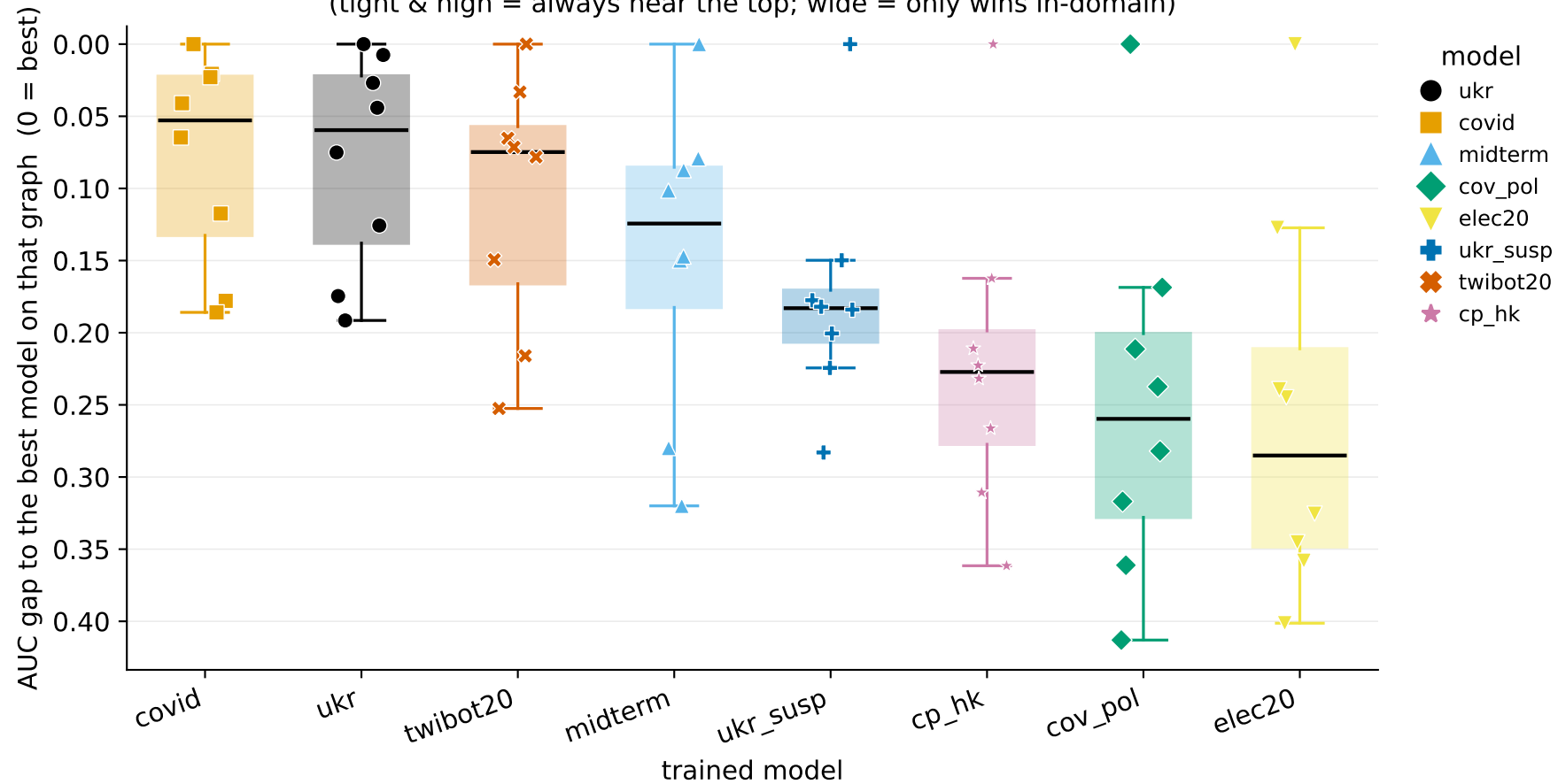
How far each model trails the best on each test graph (tight & high = always near the top; wide = only wins in-domain)
