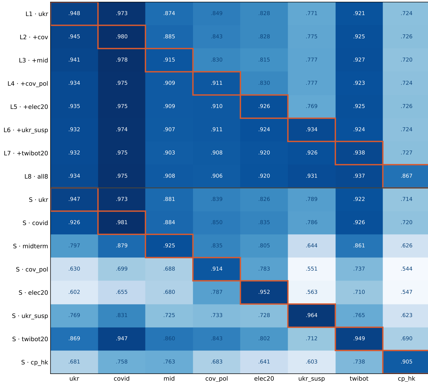
NM AUC — ladder rungs (top) + single-source specialists (bottom) coral = own-graph cell (enters merge / in-domain); matched-40k, 1 seed
