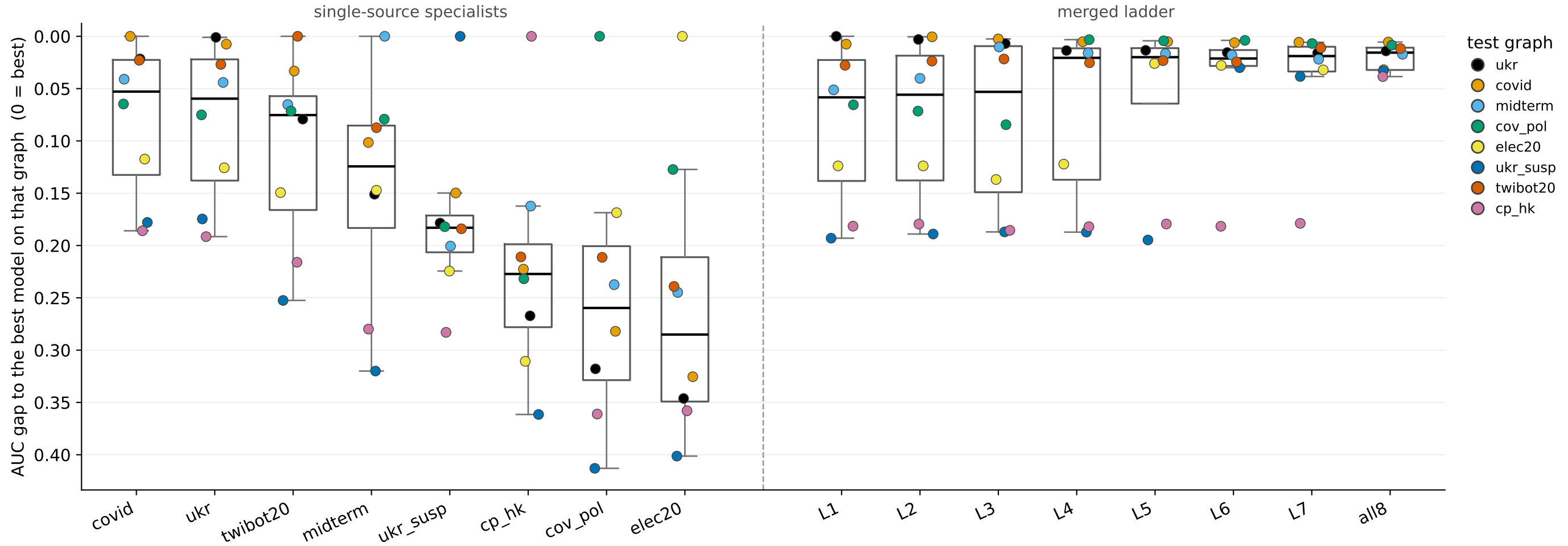
How far each model trails the best on each test graph — specialists vs ladder (best over all 16 models; single-source sorted by mean gap \uparrow ; ladder L1 \rightarrow all8; 1 seed)
